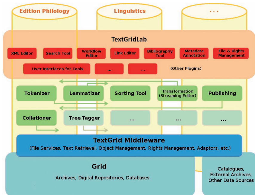
Figure 2: TextGrid architecture
